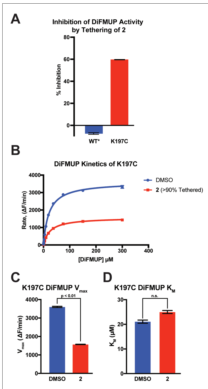
Figure 8—figure supplement 3. 2 inhibits K197C catalysis of DiFMUP through a reduction in V_{\text{max}} .
