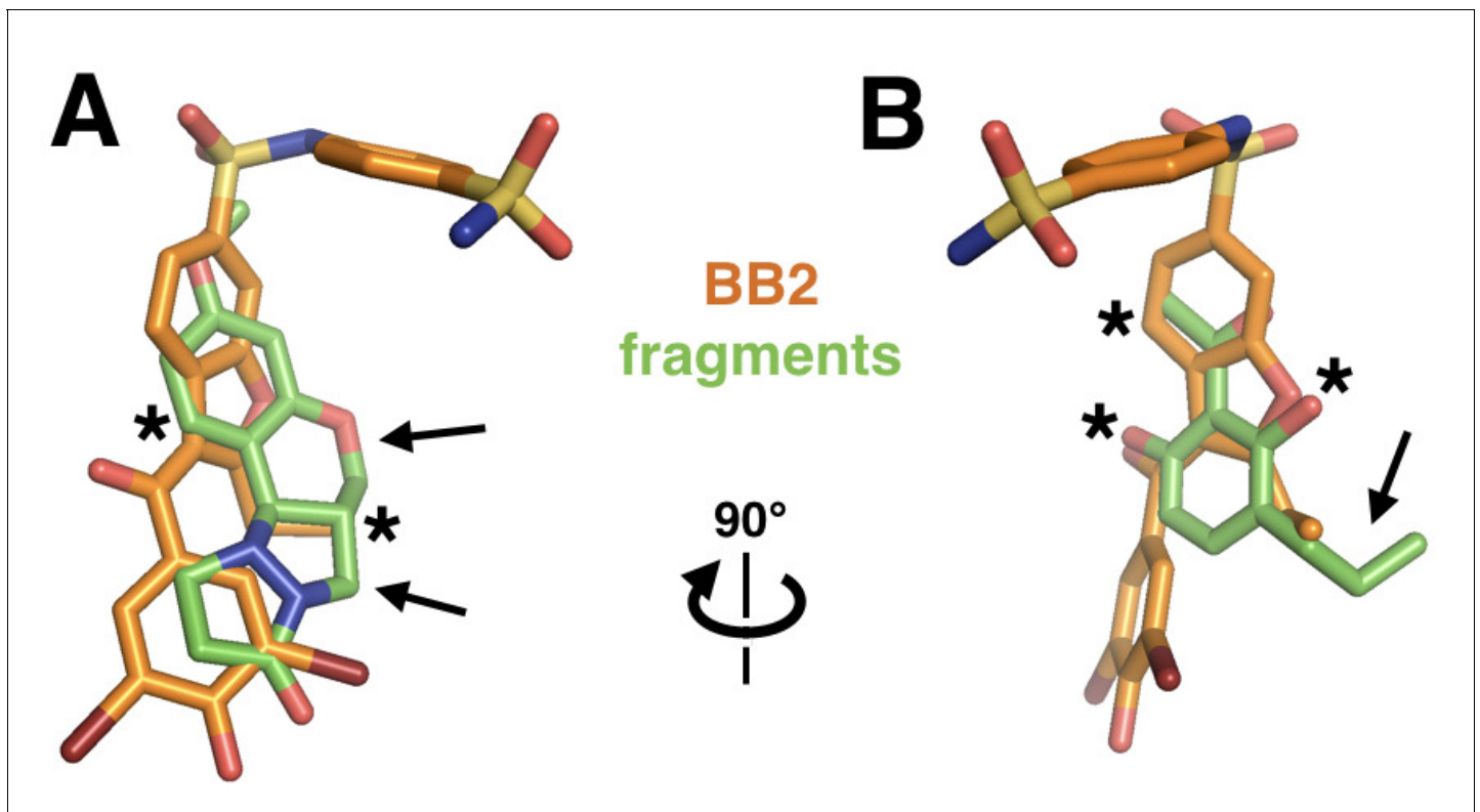
Figure 7—figure supplement 1. Fragments overlap with the BB allosteric inhibitor scaffold and suggest possible improvements. Out of the 24 fragments that bind in the same site as BB2 (PDB ID 1t49, orange), two example fragments (green) are shown that overlap parts of BB2's pose (asterisks), but also have chemical extensions that may be fruitfully added to the BB scaffold (arrows). (A) The first fragment has aromatic rings in roughly the same positions as does BB2 and a carbon matching a methyl extension in BB2, but in the fragment that carbon is part of two additional protruding rings. (B) The second fragment places two oxygens and a methyl in the same position as the equivalent atom types in BB2, but has a unique ethyl extension.
