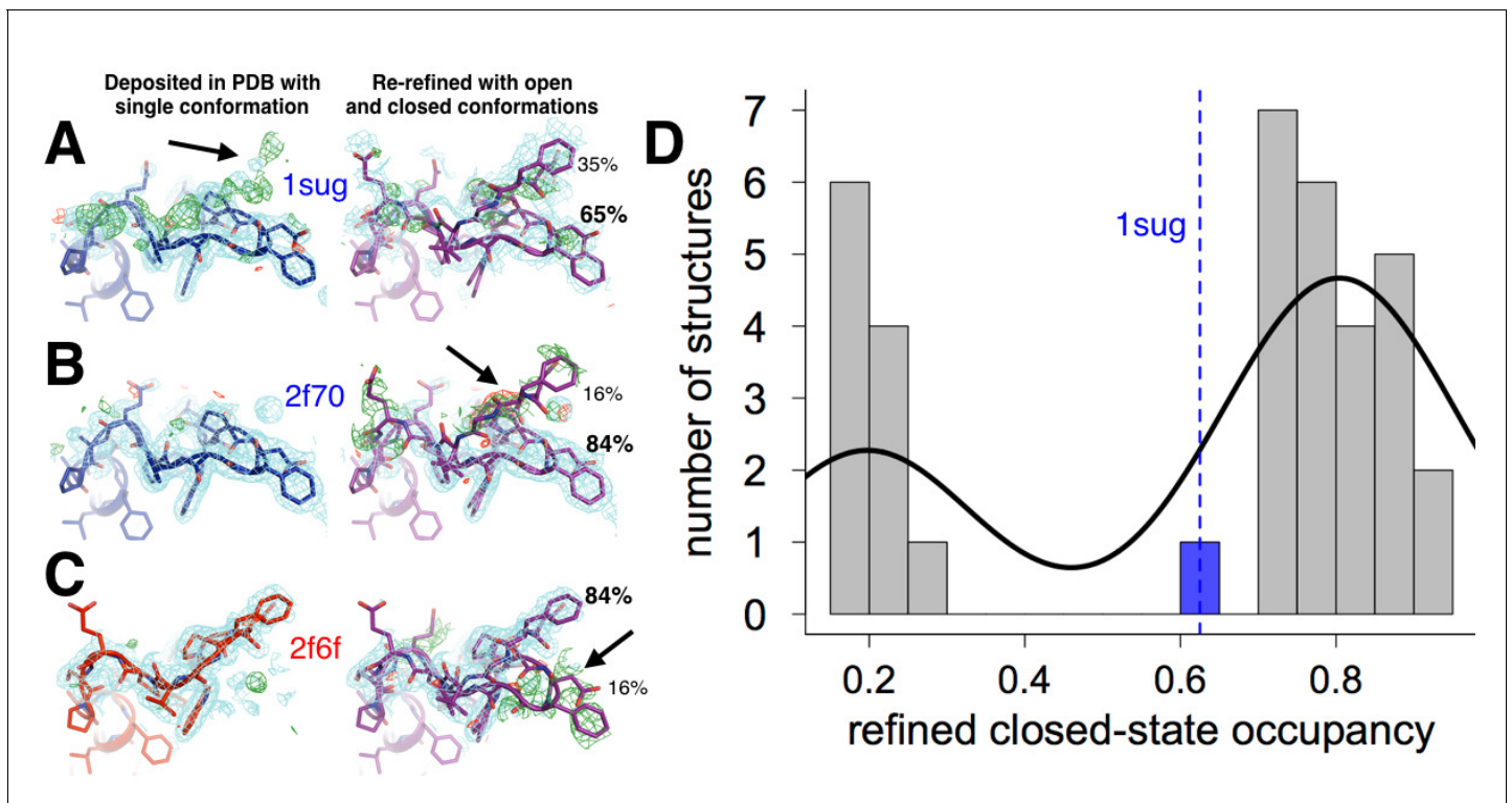
Figure 2—figure supplement 1. The WPD loop adopts multiple conformations only in the absence of inhibitors. 36 structures from the PDB in the same space group as our datasets (P3 1 21), originally modeled as only-open or only-closed, were naively re-refined with open and closed WPD loops modeled as alternative conformations with occupancies constrained to sum to 1. Almost all models have an active-site inhibitor bound. In P3 1 21 the loop is free from any crystal contacts. (A–C) Representative examples of structures with the WPD loop originally modeled as closed or open (left, blue or red), and our re-refined dual-conformation models (right, purple). 1.0 \sigma 2Fo-Fc (cyan) and \pm 3.0 \sigma Fo-Fc electron density (green/red) are shown. (A) PDB ID 1sug: apo PTP1B; originally closed. 2Fo-Fc electron density supports the dual-conformation model; residual Fo-Fc density reflects partial-occupancy waters ( Figure 2—figure supplement 2 ). (B) PDB ID 2f70: PTP1B in complex with an active-site inhibitor; originally closed. Fo-Fc electron density suggests the dual-conformation model is a poor fit. (C) PDB ID 2f6f: PTP1B in complex with another active-site inhibitor; originally open. Fo-Fc electron density suggests the dual-conformation model is a poor fit. (D) Loop occupancies for the re-refined dual-conformation models are bimodal: either ~fully open (left) or ~fully closed (right). The curve is a fit to the histogram using kernel density estimation, and is shown to emphasize the bimodal nature of the distribution. The only exception is the one published apo structure in this space group (1sug), which can be successfully refined with partial open and closed occupancies. The viewing orientation in (A–C) is as in Figure 1A ('front side' of PTP1B), except zoomed in on the active site (labeled in Figure 1A ).
