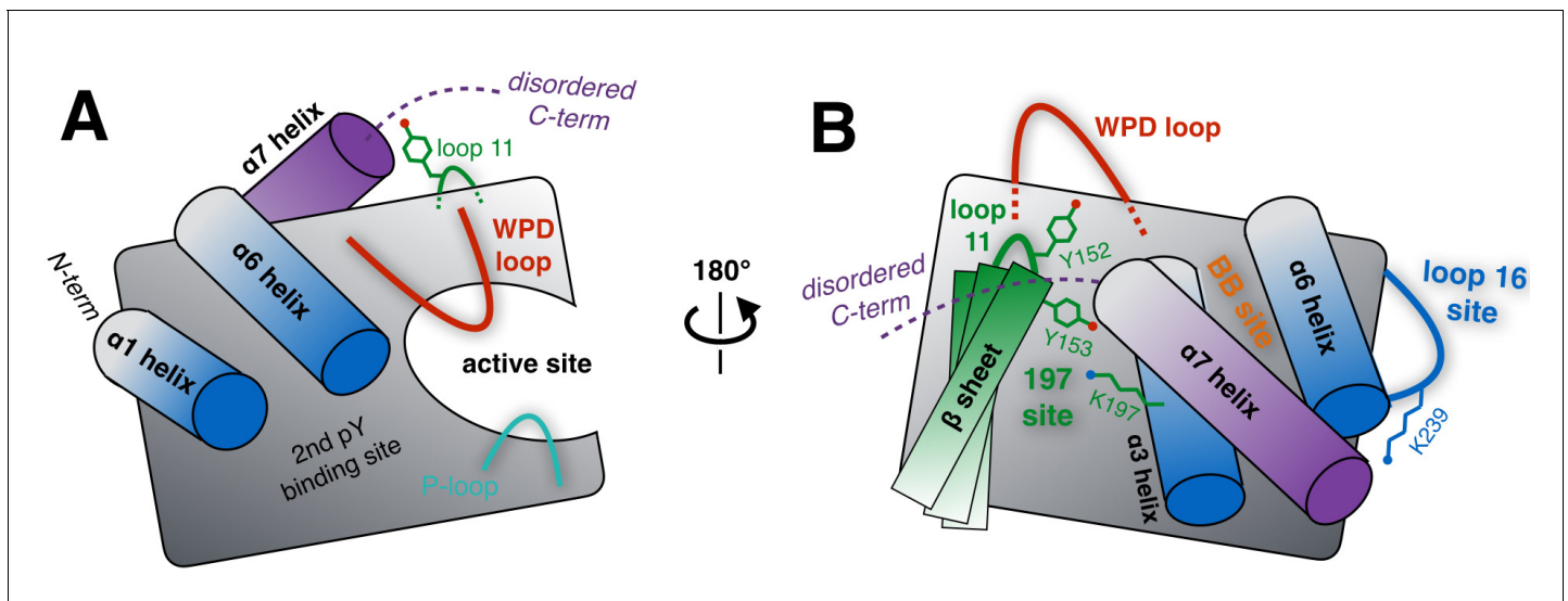
Figure 1. Schematic of key structural components in PTP1B. (A) The ‘front side’ of PTP1B features the active site covered by the dynamic catalytic WPD loop, as well as several other structural elements relevant to substrate recognition and binding. The \alpha 6 helix next to the WPD loop leads into the \alpha 7 helix and disordered C-terminus, which are positioned near loop 11 (partially occluded in this view). (B) On the ‘back side’ of PTP1B, with the view rotated by roughly 180^\circ , the \alpha 7 helix and disordered C-terminus sit atop the \alpha 3 helix, the \alpha 6 helix, and the edge of the central \beta sheet including loop 11. The pocket between the \alpha 3 helix and the \beta sheet includes several sidechains which interact with each other, leading to the ‘197 site’ (green). Elsewhere on the back side, a sidechain in loop 16 interacts with the \alpha 6 - \alpha 7 connection to form the ‘loop 16 site’ or ‘L16 site’ (blue). These two allosteric sites are distinct from the previously established ‘BB site’ (orange) (Wiesmann et al. , 2004), which is underneath the \alpha 7 helix that is displaced by BB allosteric inhibitor binding. As PTP1B transitions between its global states, many of the key structural components illustrated here undergo coordinated conformational changes, which together define the protein’s intrinsic allosteric circuitry.
