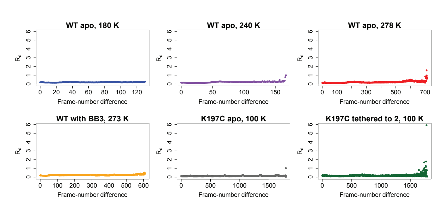
Figure 2—figure supplement 3. Radiation damage is minimal across all datasets. Plots of R_d (Diederichs, 2006) versus frame-number difference for each dataset reveal little evidence for radiation damage. Statistics for WT apo at 100 K, which is from PDB ID 1sug, are not shown.
