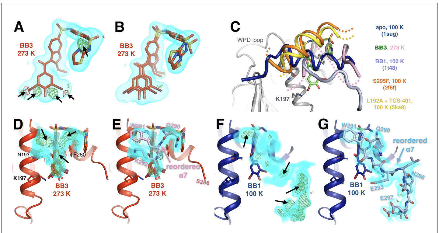
Figure 3—figure supplement 3. Allosteric-inhibitor-bound PTP1B has some low-occupancy conformations only at 273 K. (A) At 273 K, despite a good fit to 2Fo-Fc electron density, shown contoured at 0.75 \sigma (cyan volume), the allosteric inhibitor BB3 cannot be sufficiently modeled with a single conformer, as evidenced by +3.5 \sigma (green mesh) and -3.5 \sigma (red mesh) Fo-Fc difference electron density. These features are absent from the 100 K structure with BB3 (1t4j). (B) These unexplained difference features disappear when a second alternate conformer is added with a translation at the 'bottom' of the molecule (from this viewing angle) and dihedral-angle changes at the 'top right'. (C) The disordered \alpha 7 helix is reordered above the BB binding site in various structures: 273 K with BB3 (pink; BB3 molecule in green), 100 K with BB1 (pale blue, PDB ID 1t48), 100 K with the S295F mutation (orange, PDB ID 2f6f), and 100 K with the L192A mutation and the TCS-401 active-site inhibitor (yellow, PDB ID 5ka9). The normal ordered \alpha 7 conformation (blue, PDB ID 1sug) is shown for reference. See Figure 7A for another example of a reordered \alpha 7 conformation. (D–G) Evidence for some of the conformations in C. (D) At 273 K, 2Fo-Fc electron density contoured at 1.0 \sigma (cyan volume) and Fo-Fc difference electron density contoured at +3.5 \sigma (green mesh) and -3.5 \sigma (red mesh) suggest something remains unmodeled above the bound BB3 molecule. (E) Modeling a reordered portion of the disordered \alpha 7 helix, including Trp291 (pink), fits the 2Fo-Fc density, removes the positive Fo-Fc peaks, and has reasonable interactions with nearby sidechains on \alpha 3 (left). (F–G) At 100 K, the electron density (shown at the same contour levels) suggests a different reordered conformation of \alpha 7 above BB1 (PDB ID 1t48). Both reordered \alpha 7 conformations (D–E) vs. (F–G) place residues 290–292, including Trp291, in the same place. However, the C-terminal portion of the reordered conformation with BB1 at 100 K, including His296 (right), is sterically incompatible with the N-terminal portion of the \alpha 6 - \alpha 7 junction with BB3 at 278 K, including Ser286. Neither conformation is compatible with the electron density for the other, suggesting that differences in temperature and/or inhibitor dictate different \alpha 7 conformations. The viewing orientation in C–G) is as in Figure 1B ('back side' of PTP1B), except zoomed in on the BB site (labeled in Figure 1B ).
