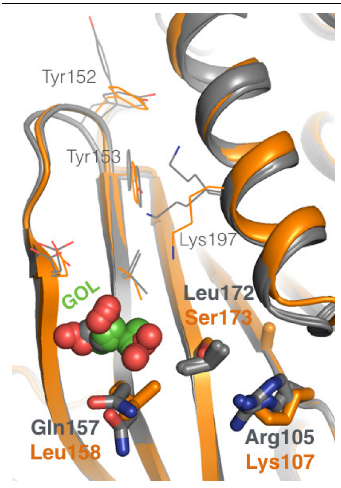
Figure 5—figure supplement 2. The allosteric 197 site has local sequence differences in related PTPs. Several amino acids in the allosteric 197 site in PTP1B (gray) are different at the equivalent positions in the closest homolog, TCPTP (orange). The viewing orientation is as in Figure 1B ('back side' of PTP1B), except zoomed in on the 197 site (labeled in Figure 1B ).
