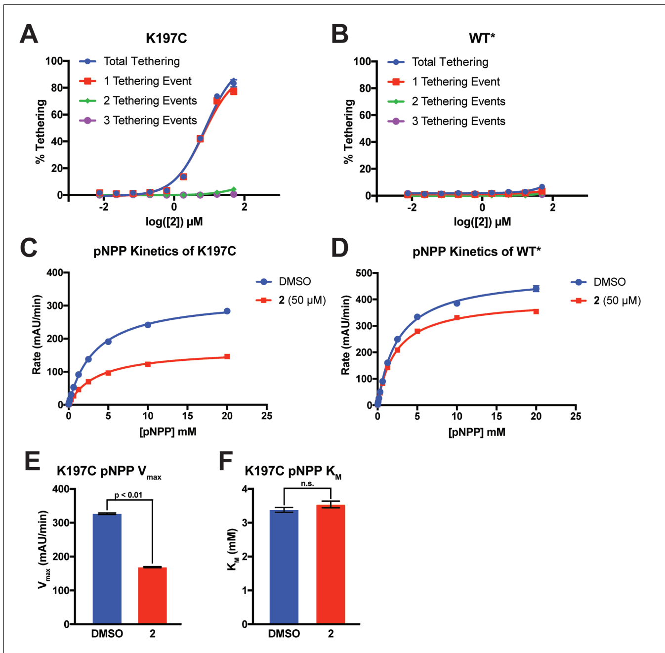
Figure 8—figure supplement 2. 2 tethers to only a single cysteine in K197C and inhibits through a reduction in V_{\text{max}} . (A) Percent tethering of K197C at varying concentrations of 2. The vast majority of labeled K197C appears to have only a single tethering event of 2, supporting specific labeling of K197C. Observation of more than one tethering event suggests nonspecific labeling of native cysteines in PTP1B. (B) Percent tethering of WT* at varying concentrations of 2. Very little tethering of WT* is observed (<10%) with the total coming from a combination of different adducts, supporting nonspecific labeling. (C) Michaelis–Menten kinetic analysis of K197C in the presence and absence of 2 (50 \mu\text{M} ). Compound 2 causes a ~54% reduction in V_{\text{max}} relative to DMSO but almost no change in K_M , supporting a non-competitive allosteric mechanism of inhibition. (D) Michaelis–Menten kinetic analysis of WT* in the presence and absence of 2 (50 \mu\text{M} ). Compound 2 causes only a ~20% reduction in V_{\text{max}} relative to DMSO but almost no change in K_M . This background inhibition does not correlate with labeling and may be caused by nonspecific factors, such as aggregation of 2 at higher concentrations ( \geq 50 \mu\text{M} ). (E) Tethering of compound 2 to K197C reduces the V_{\text{max}} observed for dephosphorylation of pNPP. Values are derived from the data shown in (C). V_{\text{max}} was calculated using the Michaelis–Menten nonlinear fit in Graphpad Prism 7. (F) Tethering of compound 2 to K197C shows no effect on the K_M observed for dephosphorylation of pNPP. Values are derived from data shown in (C). K_M was calculated using the Michaelis–Menten nonlinear fit in Graphpad Prism 7. Data represent the mean of three independent assays \pm the standard error of the mean. All p-values and significance was calculated using a FDR-Approach Multiple t-test in Graphpad Prism 7. All assays were performed in the presence of 100 \mu\text{M} of \beta -mercaptoethanol. DOI: https://doi.org/10.7554/eLife.36307.034
