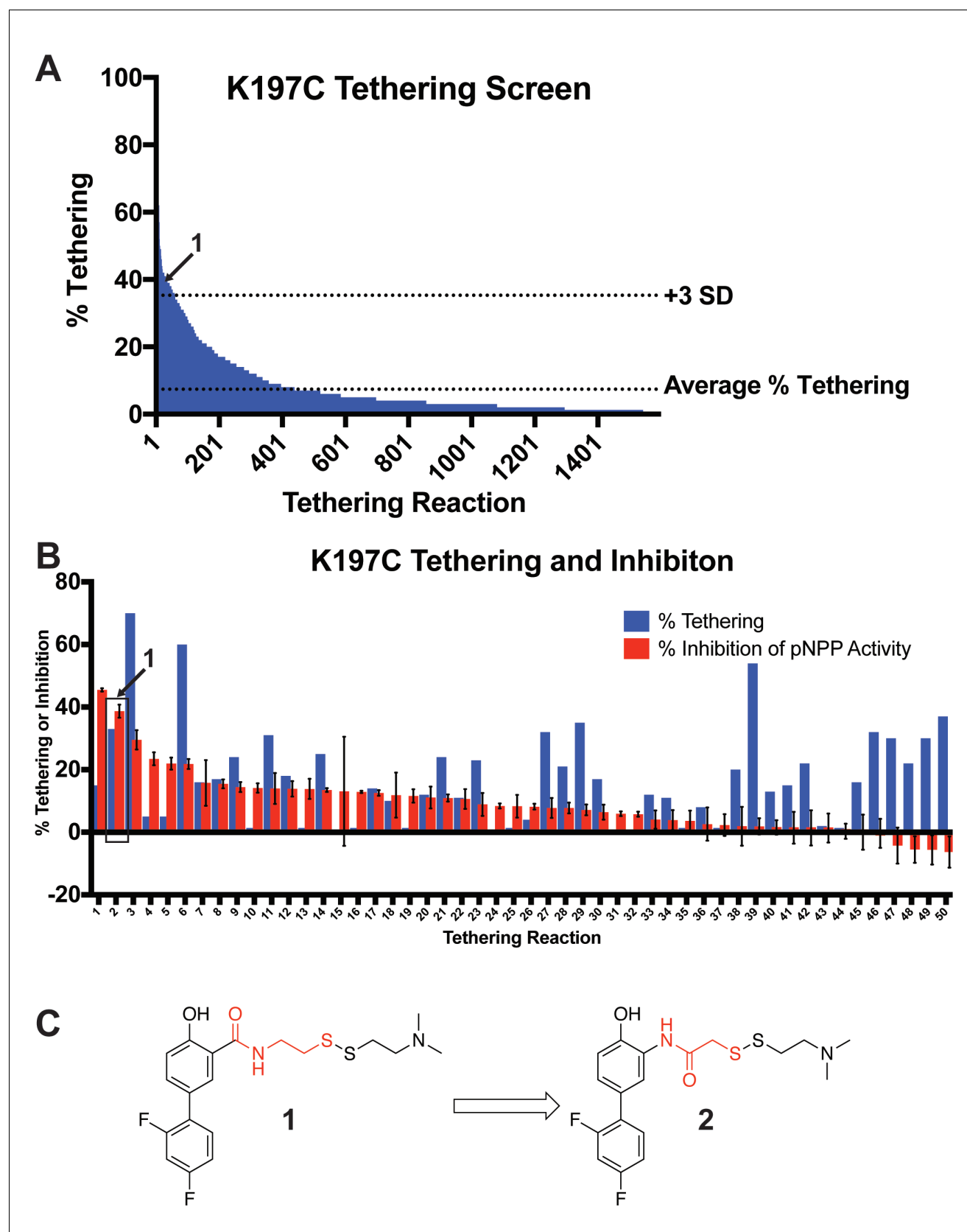
Figure 8—figure supplement 1. Identification of a functional covalent allosteric inhibitor. (A) 1600 disulfide fragments were screened for their ability to covalently label K197C. The location of 1 in the data is highlighted. Data represents a single experiment. The % Tethering data reported is for the 1:1 Figure 8—figure supplement 1 continued on next page
