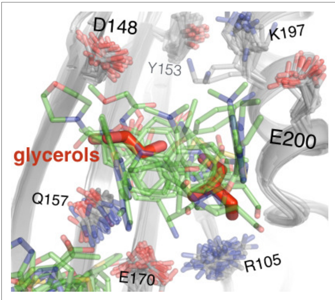
Figure 7—figure supplement 2. Fragments in the 197 site overlay with glycerols from multitemperature structures. Fifteen fragments (green) in the primary subsite of the 197 site occupy a similar region of space as ordered glycerols (red) from our 278 K apo structure. The viewing orientation is as in Figure 1B ('back side' of PTP1B), except zoomed in on the 197 site (labeled in Figure 1B ). See also Figure 6E (right) for orientation.
