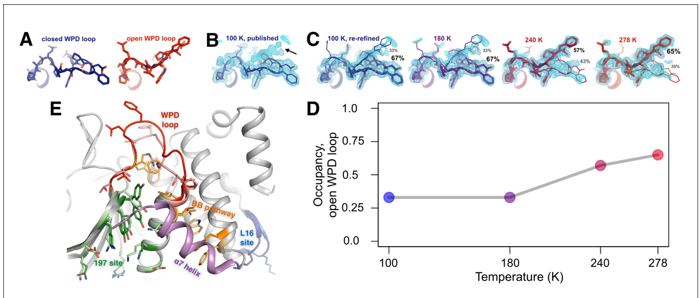
Figure 2. The conformational ensemble of the active-site WPD loop and allosterically coupled regions. (A) The active-site WPD loop in PTP1B adopts either a closed conformation (example from PDB ID 1sug) or an open conformation (example from PDB ID 1t49). View from the ‘front side’ of PTP1B. (B) In the previously published apo structure of PTP1B, solved at 100 K (PDB ID 1sug), 0.8 \sigma 2F_o - F_c electron density (cyan) supports the modeled closed conformation, but substantial electron density remains unexplained (arrow). (C) Adding the open conformation of the WPD loop as a secondary conformation at partial occupancy accounts for this electron density. In structures solved at different elevated temperatures, electron density for the open conformation becomes more prominent as its occupancy (labeled) relative to the closed conformation increases. (D) The occupancy of the open conformation increases non-linearly with temperature. (E) Overall roadmap of allostery on the ‘back side’ of PTP1B, with the allosteric 197 site and loop 16 (L16) site highlighted in the context of the larger allosteric network including the previously established BB site, \alpha 7 helix, and WPD loop. Sidechains are shown in stick representation for several key residues in the WPD loop and allosteric regions. For those residues with alternative conformations at 278 K, both open-state (darker hues) and closed-state (lighter hues) conformations are shown. The viewing orientation in (A–C) is as in Figure 1A (‘front side’ of PTP1B), except zoomed in on the active site (labeled in Figure 1A ). The viewing orientation in (E) is as in Figure 1B (‘back side’ of PTP1B).
