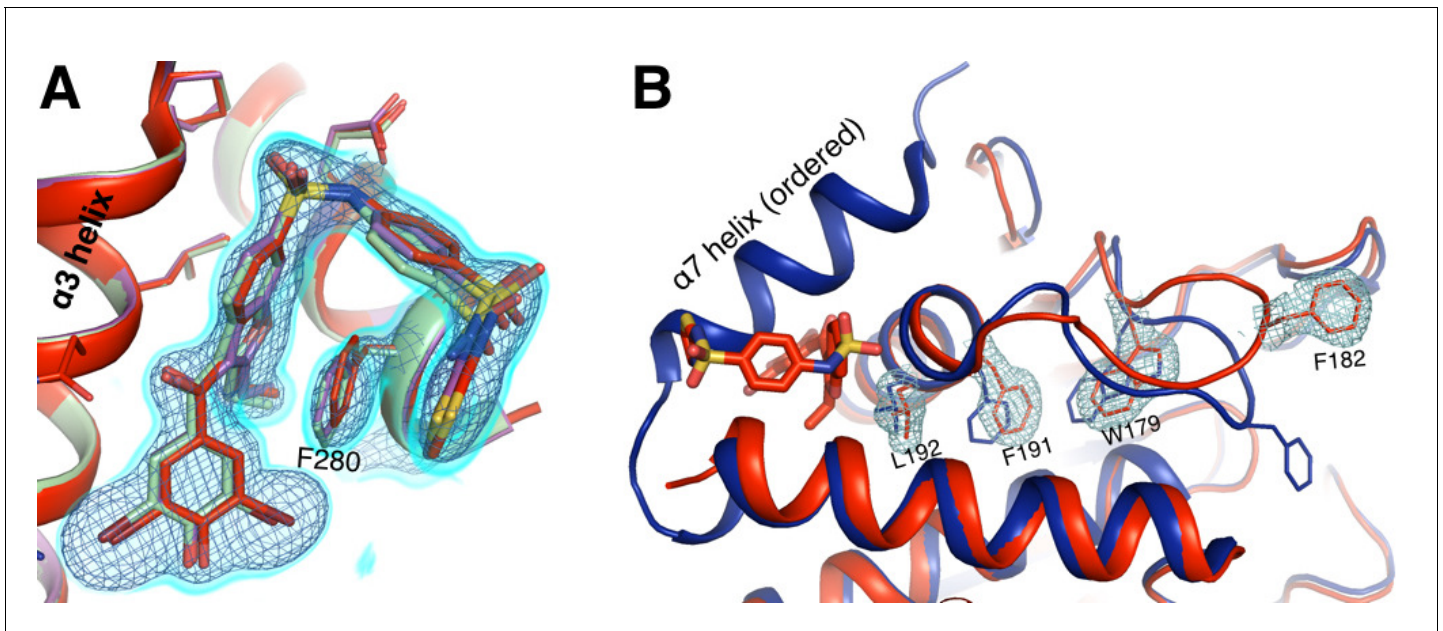
Figure 3—figure supplement 2. Allosteric inhibitor binding quenches conformational heterogeneity regardless of temperature. (A) The pose of BB3 in our new 1.80 Å 273 K structure (red) is well-justified by 2Fo-Fc electron density contoured at 0.75 \sigma (cyan volume) and at 1.5 \sigma (blue mesh). The pose is also essentially identical to the poses in previously published 100 K structures with BB3 (1t4j, magenta) and BB2 (1t49, pale green), which is very similar in structure and inhibition to BB3 (Wiesmann et al. , 2004). (B) 2Fo-Fc electron density contoured at 0.75 \sigma (cyan) supports only a single conformation along the previously characterized allosteric pathway, rather than the multiple conformations seen at 278 K from our multitemperature apo PTP1B series (Figure 3); a 100 K structure in the closed state (1sug, blue) is shown for comparison. This confirms that inhibitor binding quenches conformational heterogeneity essentially completely, locking the protein in the open state. The viewing orientation in A is as in Figure 1B ('back side' of PTP1B), except zoomed in on the BB site (labeled in Figure 1B). The viewing orientation in B is as in Figure 1A ('front side' of PTP1B), except slightly zoomed in.
