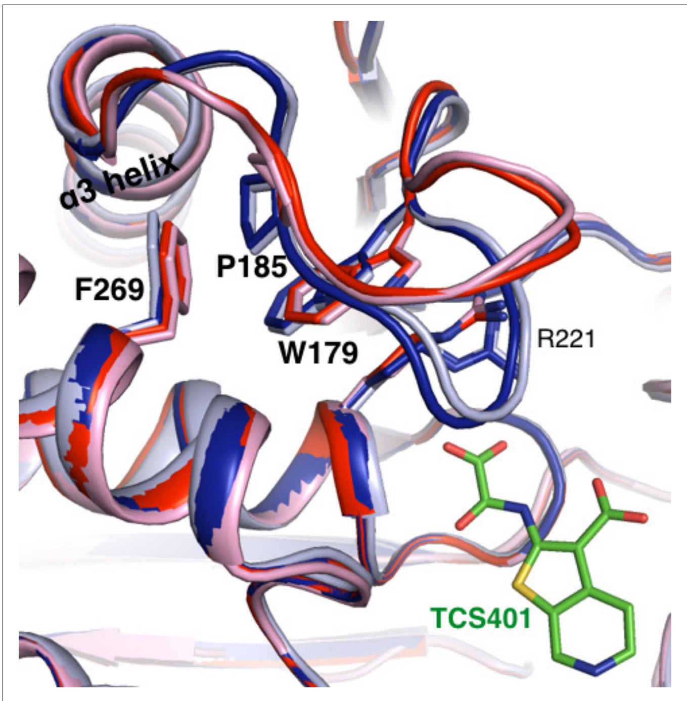
Figure 3—figure supplement 1. Alternative conformations in apo PTP1B recapitulate a reported conformational switching mechanism in the active site during WPD loop closing. Alternative conformations in our 278 K apo structure corresponding to the open state (red) vs. closed state (dark blue) recapitulate conformational changes for several residues (labeled) in the active site that undergo a CH/ \pi -mediated switch between the open state (pink, 5k9v) and TCS401-inhibitor-bound closed state (light blue, 5k9w) (Choy et al., 2017). The viewing orientation is as in Figure 1A ('front side' of PTP1B), except zoomed in on the active site (labeled in Figure 1A ).
