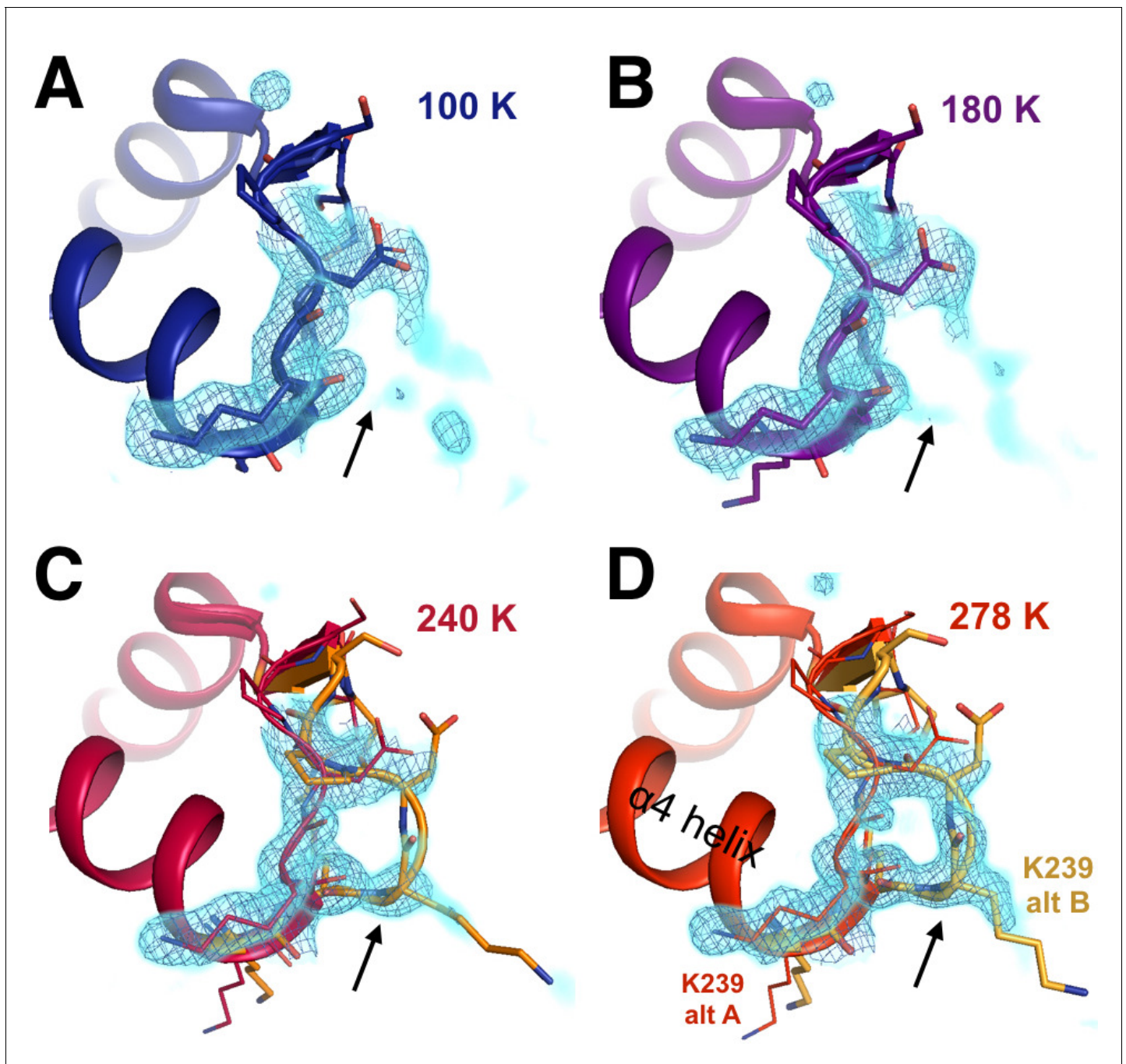
Figure 4—figure supplement 1. The conformational distribution of the \alpha 7 -coupled loop 16 titrates with temperature. The loop consisting of residues 237–243 (bottom right) is single-conformer at low temperatures including (A) 100 K and (B) 180 K, as evidenced by 2Fo-Fc electron density contoured at 1.0 \sigma (cyan volume) and at 1.0 \sigma (blue mesh). By contrast, it adopts multiple conformations at higher temperatures including (C) 240 K and (D) 278 K. The viewing orientation is as in Figure 4 .
