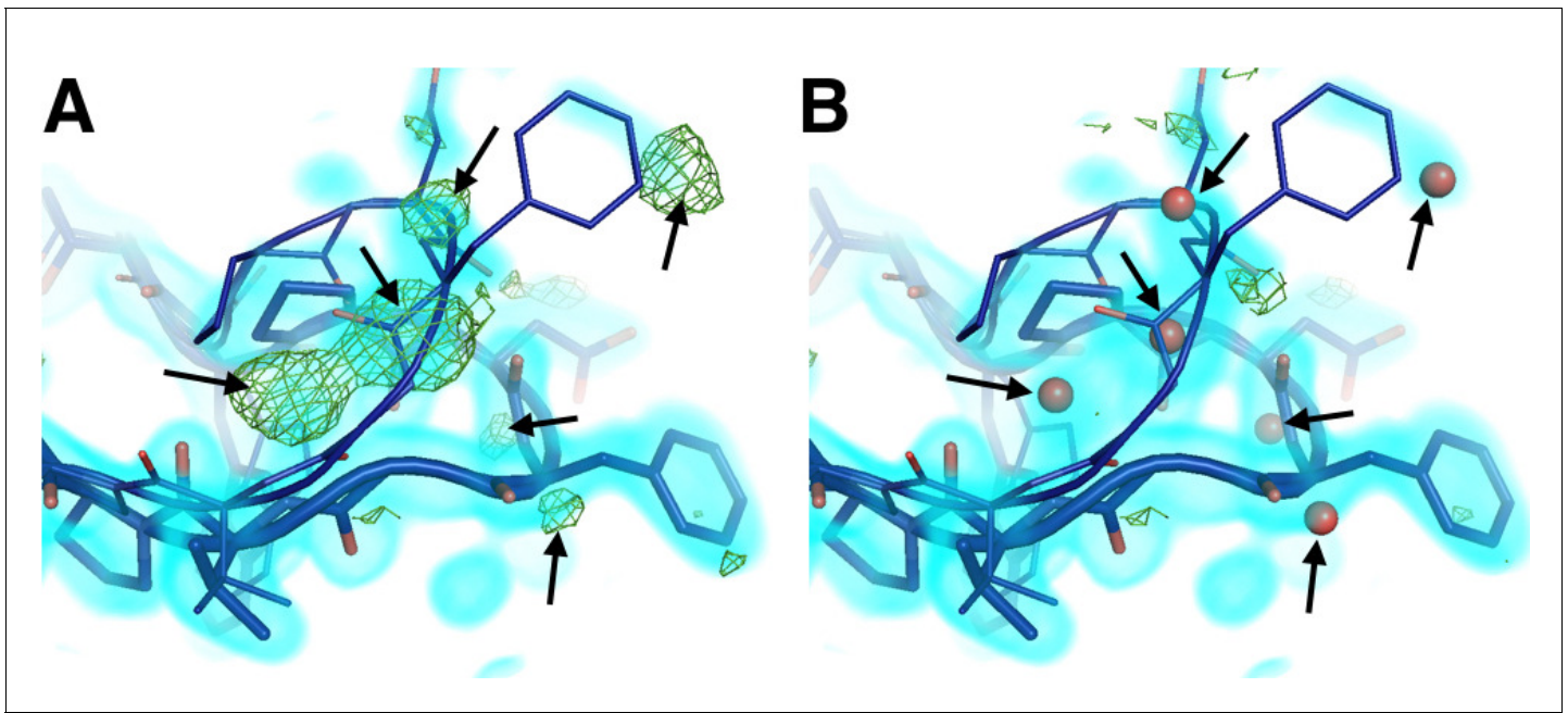
Figure 2—figure supplement 2. Mutually exclusive partial-occupancy protein and solvent atoms complicate model building. (A) Although both closed and open WPD loop states are supported by 0.8 \sigma 2Fo-Fc electron density (cyan volume) in the 100 K apo PTP1B structure, several +3.2 \sigma Fo-Fc electron density (green mesh) remain unexplained (arrows). (B) Partial-occupancy waters (red spheres) with the opposite 'altloc' alternative conformation label as the closest protein atoms ('A' vs. 'B') dramatically reduce the difference density and better explain the data. See (Pedersen et al., 2004). The waters modeled here resemble water networks from either the closed-only (2f70) or the open-only (2f6f) structures. The viewing orientation in A–C is as in Figure 1A ('front side' of PTP1B), except zoomed in on the active site (labeled in Figure 1A).
