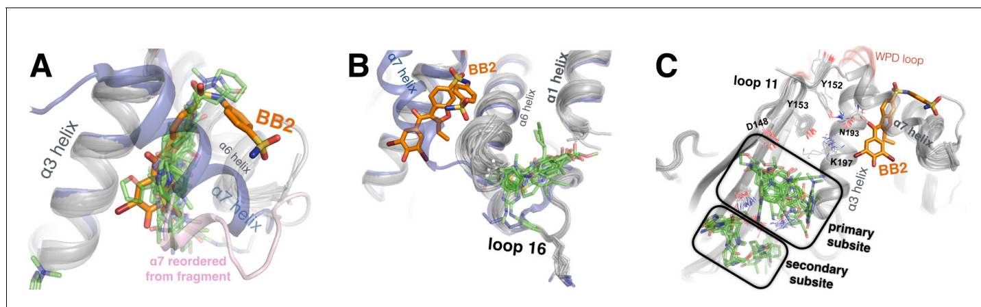
Figure 7. Fragments cluster at three binding hotspots distal from the active site. (A) Twenty-four fragments (green) bind to the same site and in similar poses as the BB2 inhibitor (orange, PDB ID 1t49), and similarly displace the \alpha 7 helix (foreground, transparent blue, PDB ID 1sug). BB2 is also shown in the following panels to emphasize that its binding site is distinct from the other fragment-binding hotspots. One structure with a fragment bound in this site features a reordered conformation of the \alpha 7 helix (pink). (B) Seventeen fragments bind to the L16 site, where they may modulate the conformations of loop 16, the \alpha 6 helix, and the protein's N-terminus on the \alpha 1 helix. (C) Thirty fragments bind to the 197 site in one primary subsite contacting K197, or a distinct secondary subsite nearby. The viewing orientation in (A) is as in Figure 1B ('back side' of PTP1B), except zoomed in on the BB site (labeled in Figure 1B ). The viewing orientation in (B) is also as in Figure 1B , except looking left from the right of that image and zoomed in on the L16 and BB site site. The viewing orientation in (C) is also as in Figure 1B , except zoomed in on the 197 site and BB site (labeled in Figure 1B ). See also Figure 6E (right) for orientation.
