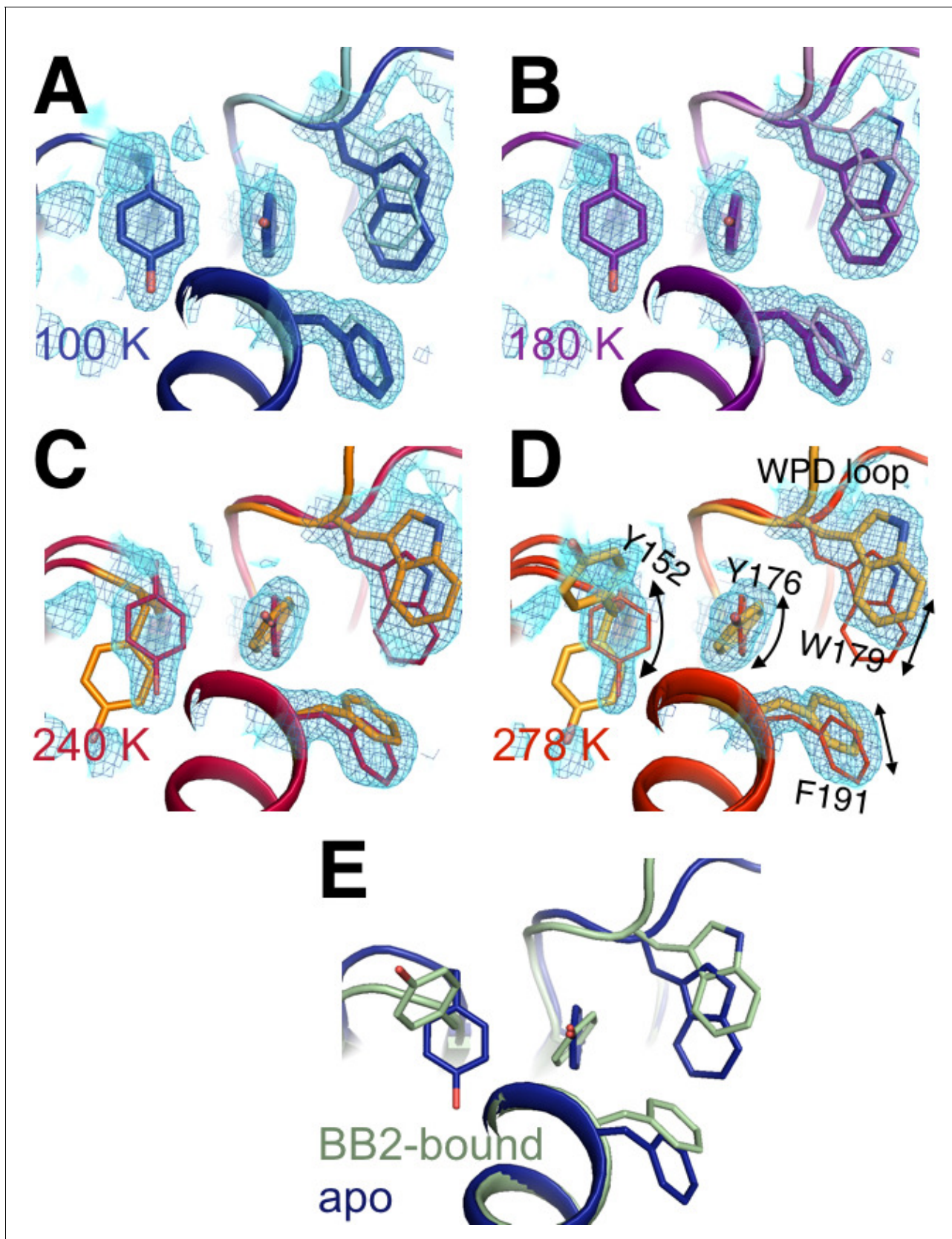
Figure 5—figure supplement 4. Flexible aromatic residues complete an allosteric circuit. Conformational heterogeneity for Tyr176 links Tyr152 in the allosteric 197 site to Phe191 in the previously reported allosteric pathway ( Wiesmann et al., 2004 ) and Trp179 in the WPD loop, thus completing an Figure 5—figure supplement 4 continued on next page
