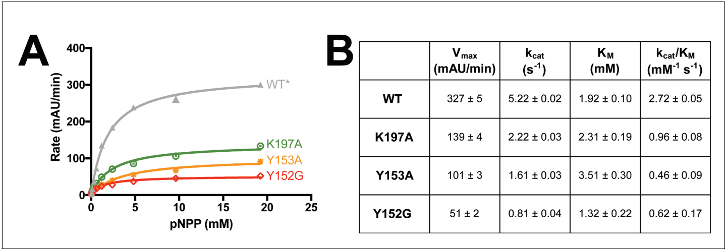
Figure 5—figure supplement 3. Mutations along the 197 site’s allosteric pathway reduce enzyme activity. (A) Point mutations to several residues along the allosteric pathway from the allosteric 197 site to the active site reduce activity to varying degrees. Data represent the mean of four independent assays ± standard deviation. (B) Michaelis-Menten kinetics for WT* vs. allosteric point mutants ± the standard error of the mean. See Materials and methods for details. DOI: https://doi.org/10.7554/eLife.36307.021
