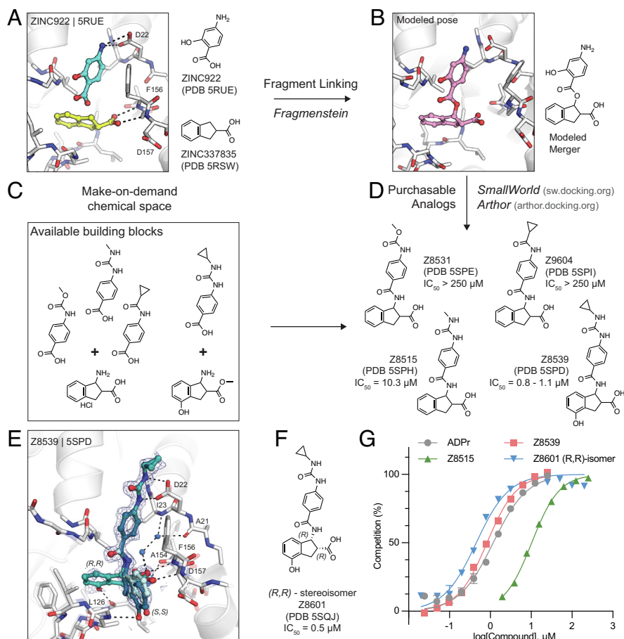
Fig. 2. In silico fragment linking targeting the adenosine site of Mac1. A ) Binding pose of two fragments identified in the previously reported fragment screen (12). Fragment protein hydrogen bonds are shown with dashed black lines. B ) Theoretical linked scaffold of ZINC922 and ZINC337835 generated using Fragmenstein . C ) Availability of corresponding chemical building blocks and reactions in the Enamine REAL database. D ) Readily accessible analogs of the theoretical scaffold shown in B . E ) X-ray crystal structure of Mac1 bound to Z8539. Three conformations of Z8539 [( R,R ) and two ( S,S )] could be resolved in the PanDDA event map (blue mesh contoured at 2 \sigma ). Water molecules that form bridging hydrogen bonds between Z8539 and the protein are shown as blue spheres. The apo state of Mac1 is shown with transparent white sticks. F ) 2D structure of the most potent ( R,R )-stereoisomer of Z8539 (Z8601). G ) ADPr-peptide competition (%) of Z8539, Z8515, and Z8601 on Mac1 determined by an HTRF-based displacement assay. ADPr was used as reference. Data are presented as the mean \pm SEM of at least two technical replicates.
