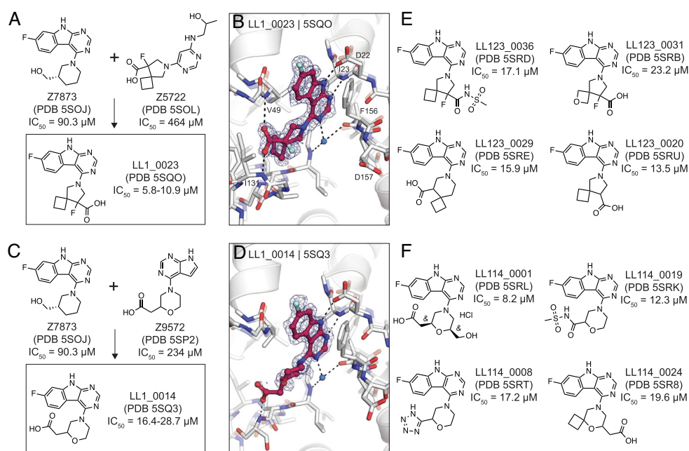
Fig. 7. Structure-based optimization of docking hits. A) Design of LL1_0023. B) X-ray crystal structure of LL1_0023. The PandDA event map is shown around the ligand (contoured at 2 σ). Hydrogen bonds are shown with dashed black lines. C and D) Design and X-ray crystal structure of LL1_0014, respectively. E and F) Selected analogs of LL1_0023 and LL1_0014, respectively.
